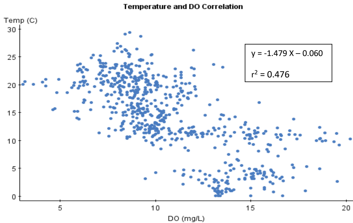
Figure 3.60. Relationship between temperature and dissolved oxygen.
