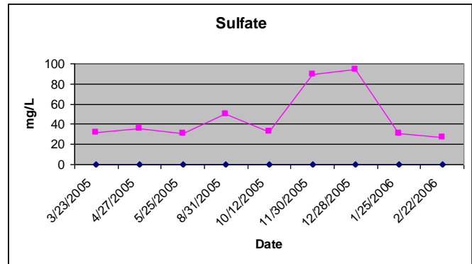
Figure 3.9 Sulfate at Site DOW05020011
