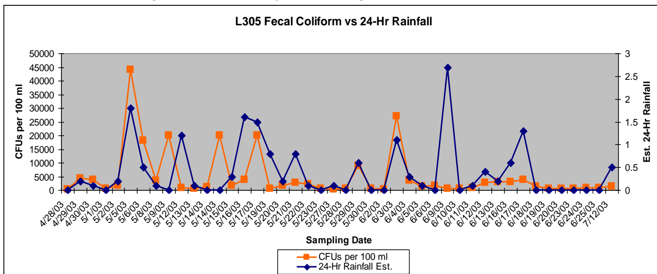
Figure 3.14: Fecal coliform data over time. Source: Tetra Tech, 2009.
