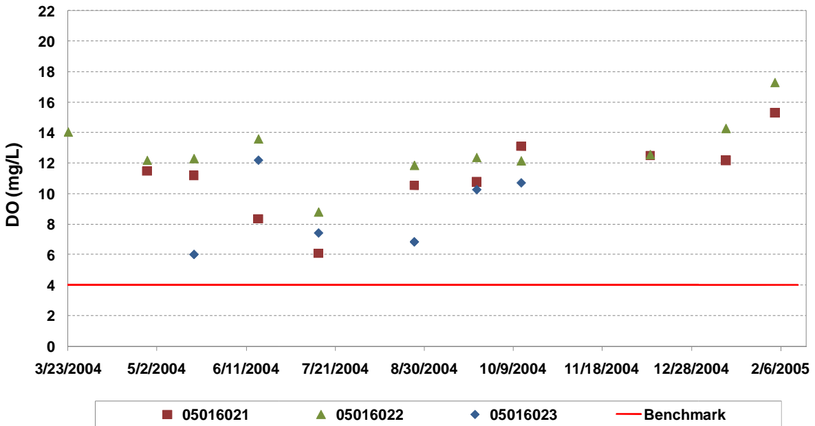
Figure D-33. Dissolved Oxygen Concentrations Measured for Tributary KDOWN Stations
