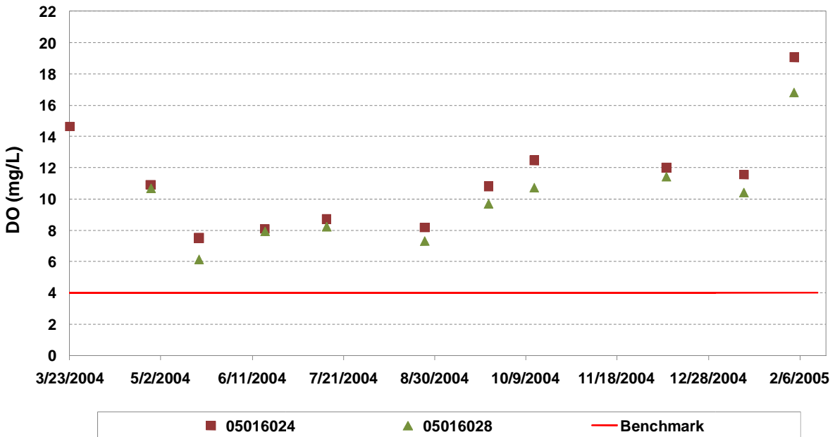
Figure D-34. Dissolved Oxygen Concentrations Measured for Tributary KDOWN Stations
